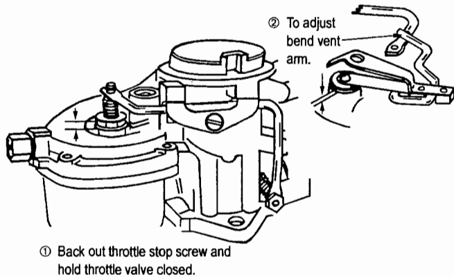
Bowl Vent Adjustment
