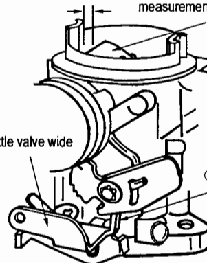
Unloader Adjustment
