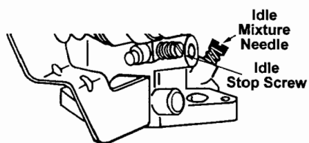
Slow Idle Adjustment
